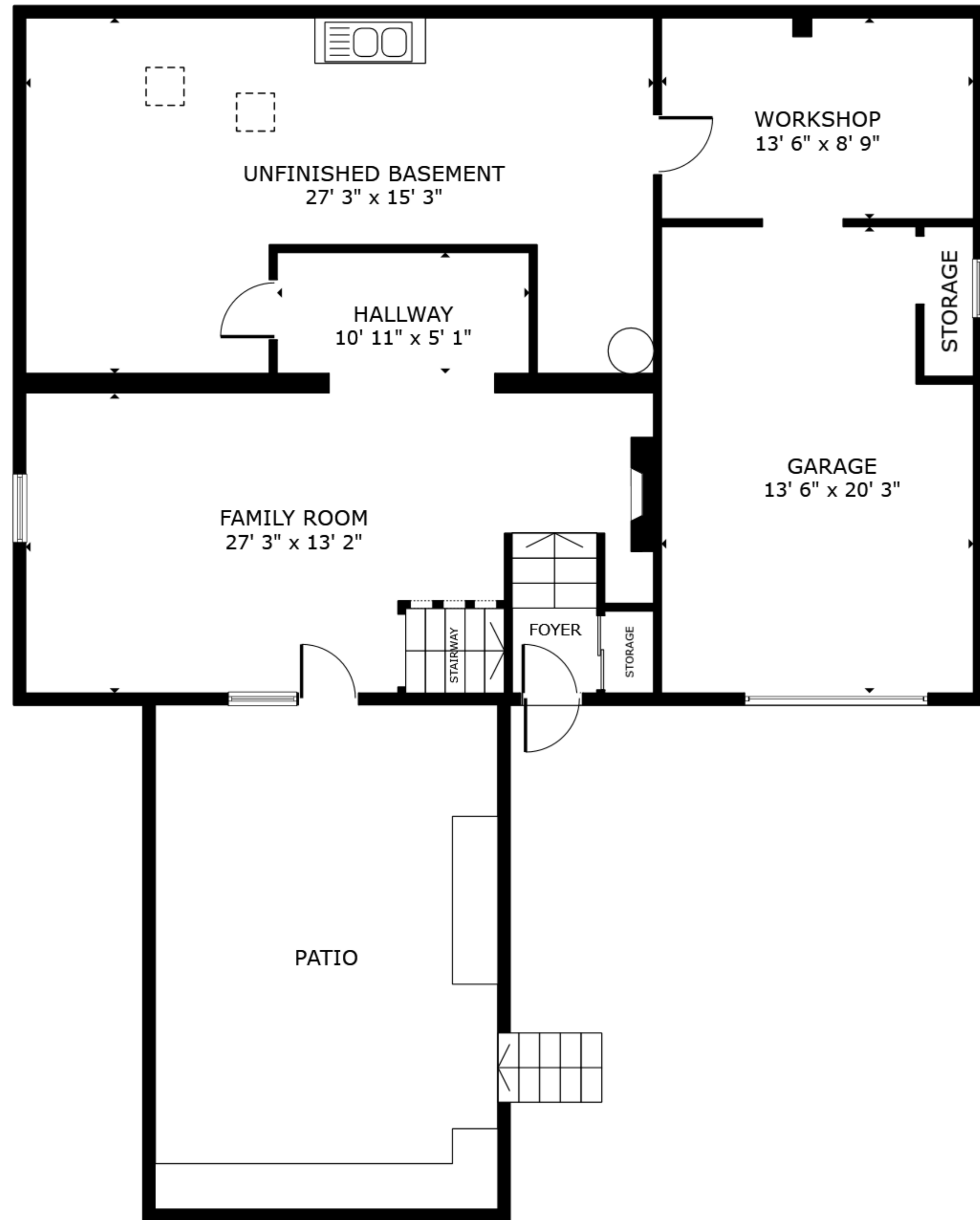
FLOOR 1
